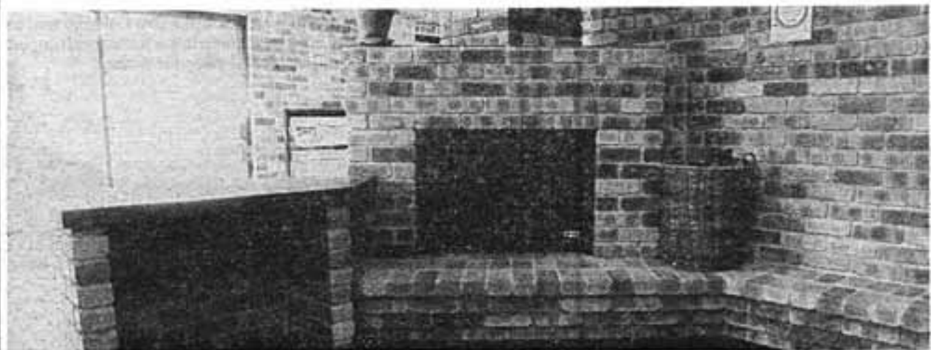
□ This ducted fireplace with its solid mass of brickwork provides a good heat storage mechanism.
